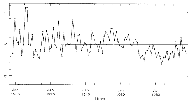
Figure 11. Northeast Brazil rainfall index (top panel) is calculated from data for Fortaleza (3.7°S, 38.5°W) and Quixeramobim (5.3°S, 39.3°W) Brazil as obtained from the NCAR World Monthly Surface Station Climatology. The Sahel series is based on an average of annual standardized anomalies from 14 stations within the region 8°–20°N and 20°W–10°E obtained from the NCAR World Monthly Surface Station Climatology
