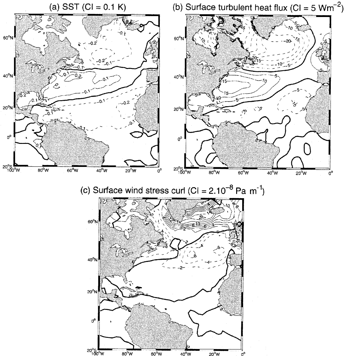
Figure 2. Regression maps of (a) SST (CI = 0.1 K, negative dashed), (b) surface turbulent heat flux (latent + sensible, CI = 5 Wm -2 , dashed out of the ocean) and (c) surface wind stress curl (CI = 2 \times 10^{-8} Pa m -1 , dashed for anticyclonic) anomalies onto the NAO index shown in Figure 1(b). The thick black line is the zero wind curl line of the climatological winds. The SST and wind stress curl data come from the NCEP–NCAR reanalysis, while the surface heat flux anomalies come from Da Silva et al. (1994). A linear trend was removed to all datasets prior to computing the linear regressions
