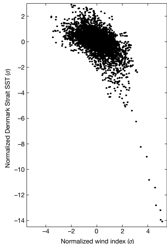
Figure 4 Scatter plot of sea surface temperature (SST) averaged over the Denmark Strait ( 62.2-66.7^\circ N, 18.8-30^\circ W) versus winds blowing perpendicular to the Denmark Strait. Before plotting, SST was made to lag the wind index by 2 yr. The ten points representing the coldest SSTs all correspond to the extreme event. The wind index is defined as the surface pressure difference between two regions: 48.9-57.8^\circ N, 33.8-56.25^\circ W (an area south of the tip of Greenland) and 66.7-75.6^\circ N, 11.3-41.3^\circ E (centred over northern Scandinavia). A Hamming 40-yr low-pass filter has been applied to the SST and wind index, and both time series have been normalized by their respective standard deviations. For clarity, only every third year of the time series is shown. The model climate exhibits a quasi-linear millennial-scale trend over the course of the 15,000-yr experiment (Fig. 1a). To ensure this model drift does not distort the distribution of variability presented here, all variations lasting longer than 1,000 yr were removed from the SST and wind index time series using a Hamming high-pass filter. The North Atlantic Oscillation index is defined as the pressure difference between two regions: 40.0-48.9^\circ N, 11.2-26.2^\circ W and 66.7-75.6^\circ N, 3.8-18.8^\circ W). Variations lasting less than 40 yr were also removed from this time series.
