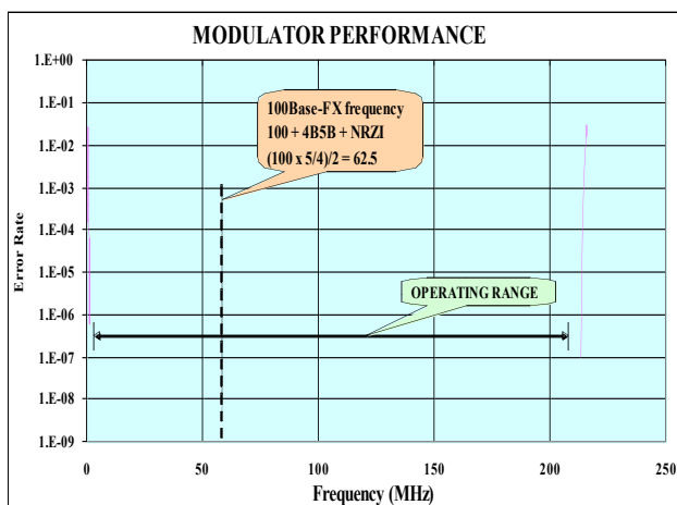
Figure 5: Modulator Performance (prototype)
