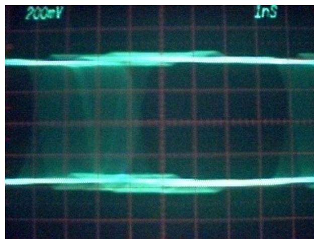
Figure 4: Measured 100Base-TX (FX) Eye Diagram
