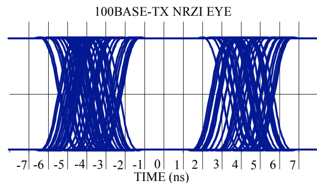
Figure 3: Simulated Sampled Data Eye Diagram
