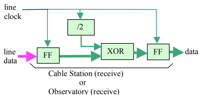
Figure 2: Data Transport De-modulator
