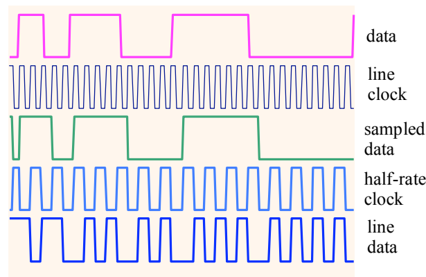
Figure 1b: Data Transport Modulator Signals
