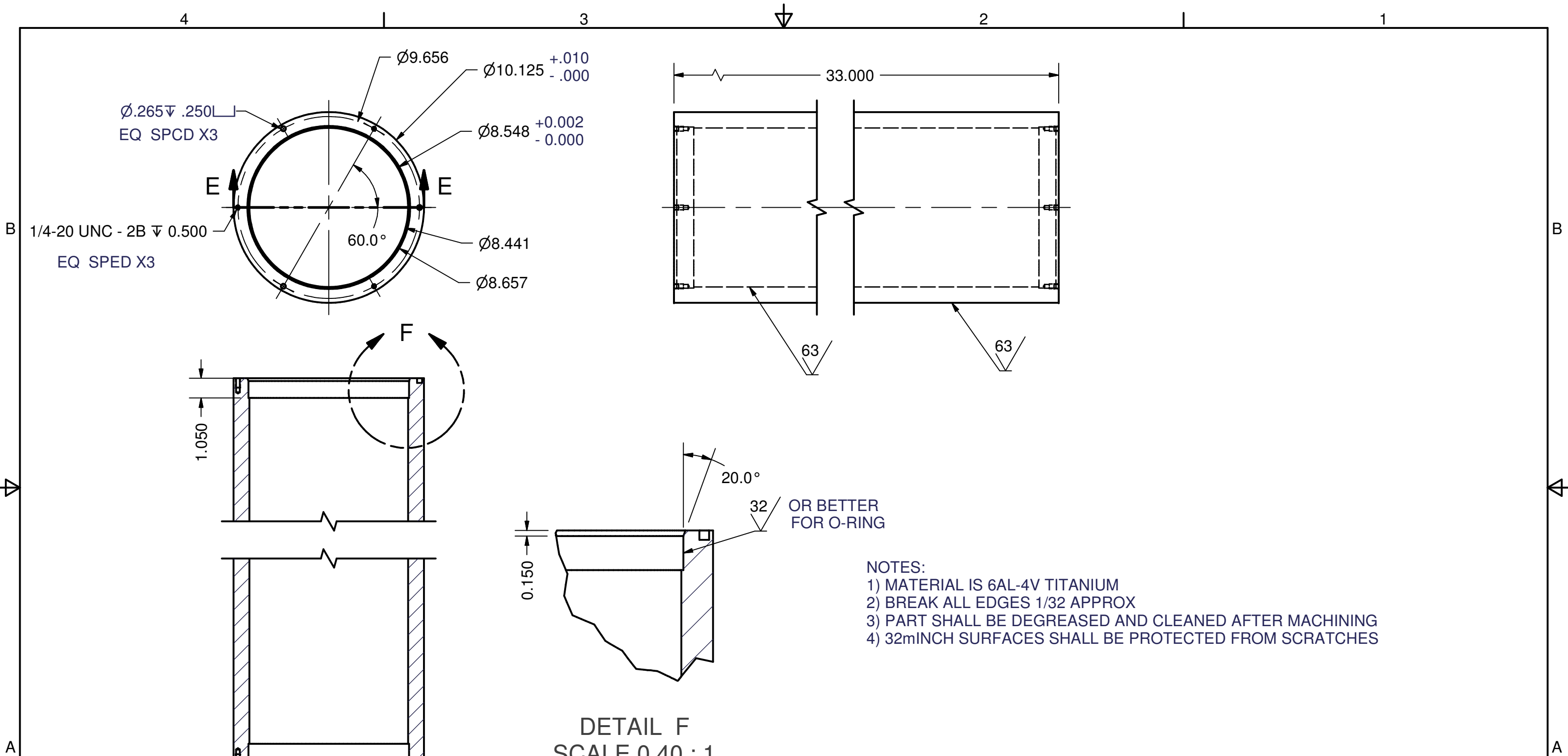
SECTION E-E SCALE 1 / 5
