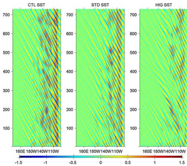
Figure 2. Filtered time-longitude SST displaying TIWs for the CTL, STD, and HIG experiments averaged over the latitudinal band from 1°N to 3°N. Units are °C.
