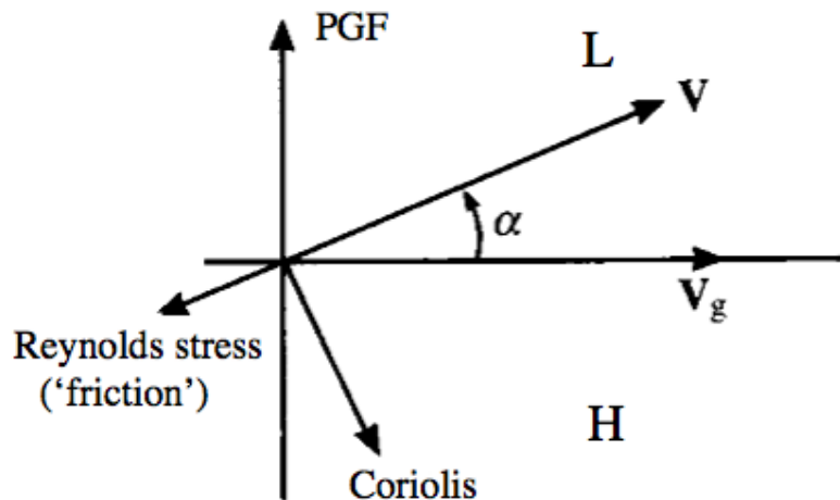
Fig. 3.1: Surface layer force balance in a steady state BL ( f > 0 ). Above the surface layer, the force balance is similar but the Reynolds stress need not be along -\mathbf{V} .
