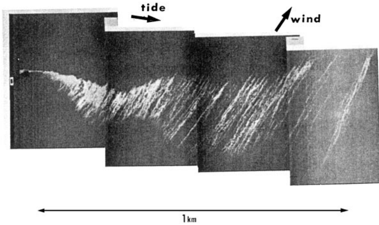
Figure 5 Spread of oil carried by a tidal flow from a fixed source at the left of the picture, a composite of infrared images taken from an aircraft. The Lc draws the oil into bands in the wind direction. The wind speed is about 10 \text{ ms}^{-1} . (Images kindly provided by Dr. T. Lunel.)
