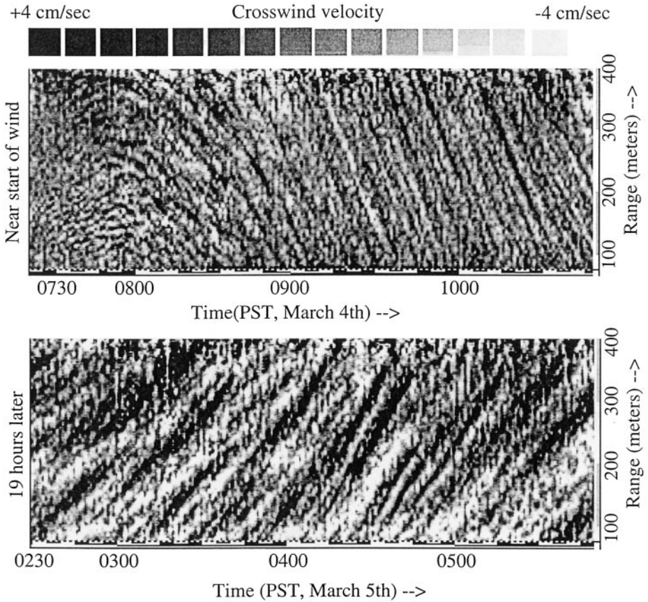
Figure 11 Near-surface convergence speed measured by Doppler sonar pointing approximately across wind. The wind increased rapidly at time = 0730 ( top ), leading to the development of a pattern of cells with gradually increasing scales that slowly drift towards the sonar. Nineteen hours later ( bottom ) the patterns show stronger flows and larger cell sizes moving away from the sonar. The near-vertical bands are caused by surface waves. (From Smith 1996.)
