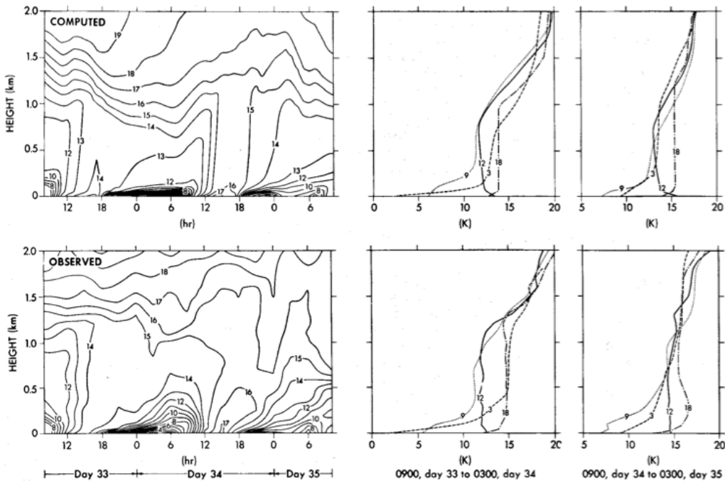
Fig. 11. Observed and calculated atmospheric boundary layer and vertical and temporal variations of mean virtual potential temperature -273°K. Units are degrees Kelvin.
