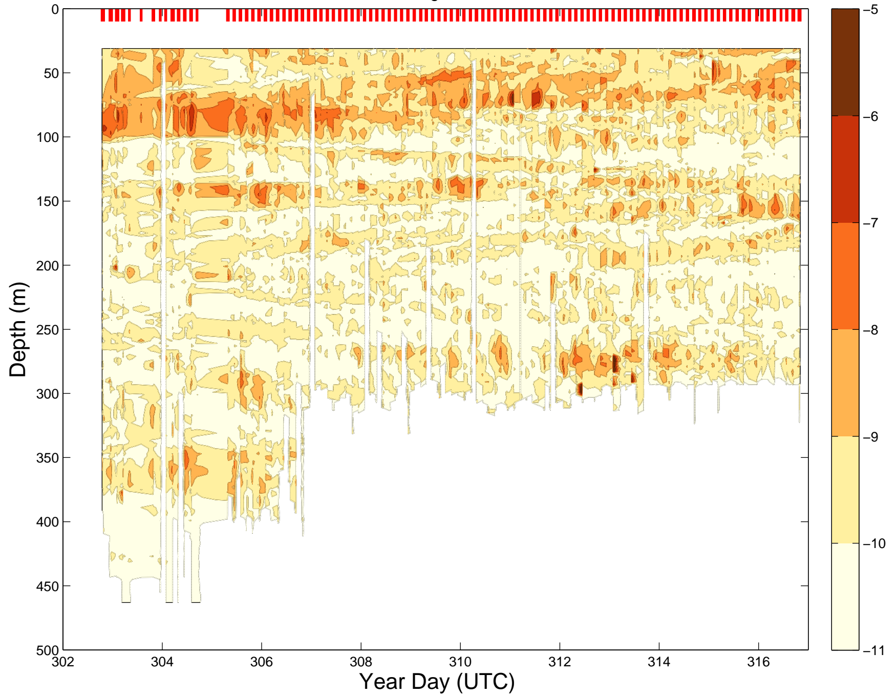
km1225: \log_{10}(\epsilon_{gc}) (equiv. depth)
