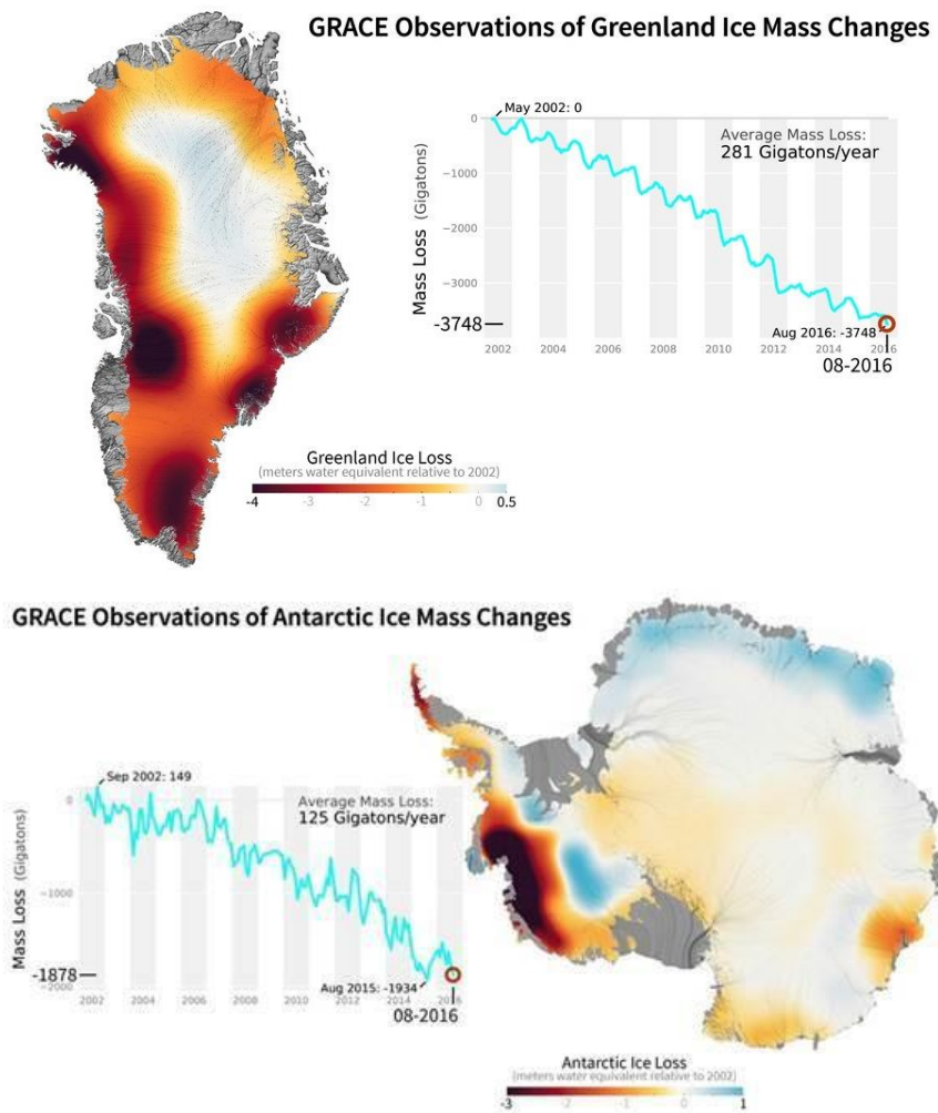
Figure 11. Ice mass loss in gigatons per year from Greenland and Antarctica (NASA 2017a)
