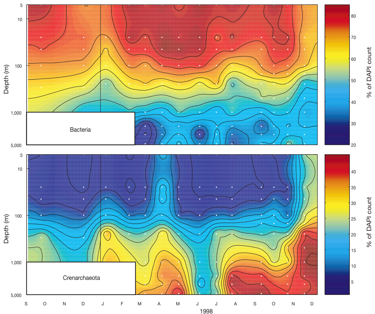
Figure 1 Contour plots of relative abundances with depth of bacteria and pelagic crenarchaeota during a 1-yr sampling effort at the Hawai'i Ocean Time-series station, ALOHA, in the North Pacific subtropical gyre. White dots indicate dates and depths where samples were collected. Contour lines are percentages of bacteria and pelagic
