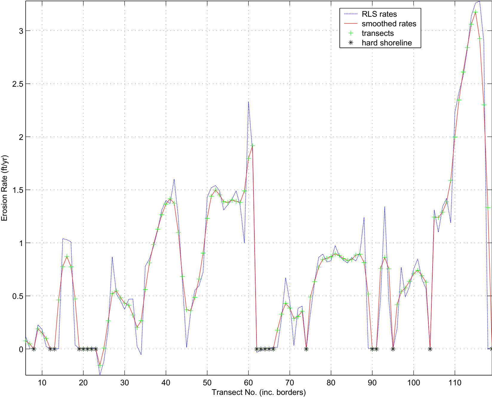
Calculated and Smoothed South Wailea Erosion Rates
