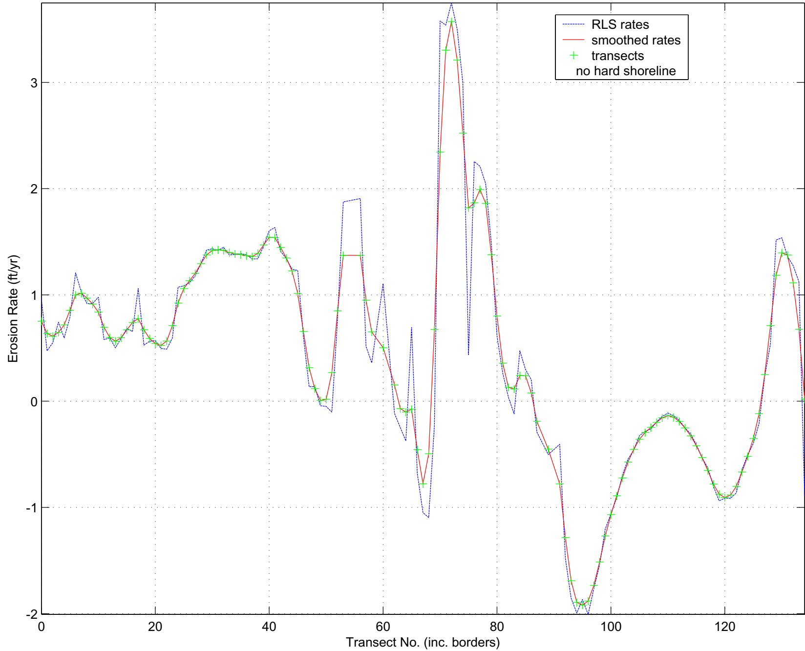
Calculated and Smoothed Puamana Erosion Rates
