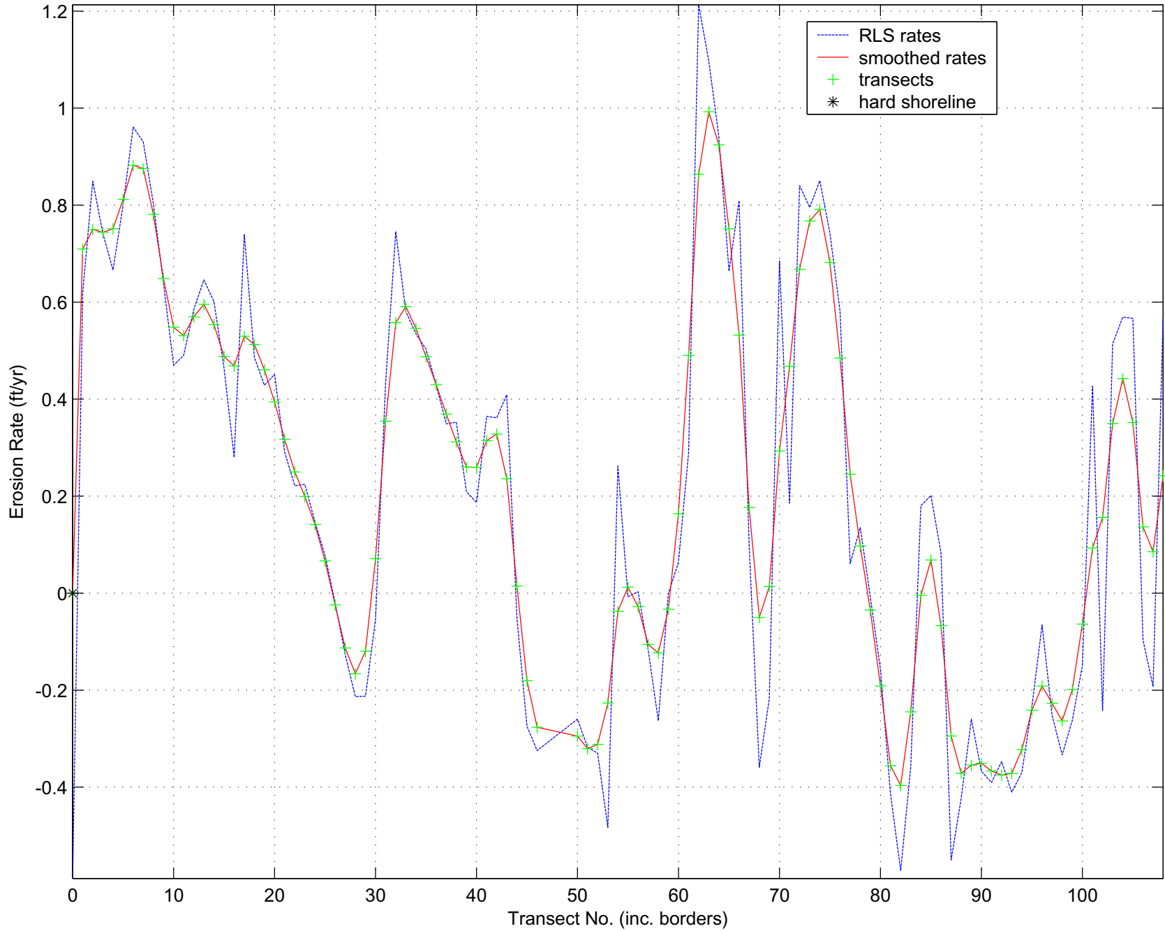
Calculated and Smoothed Olowalu Erosion Rates
