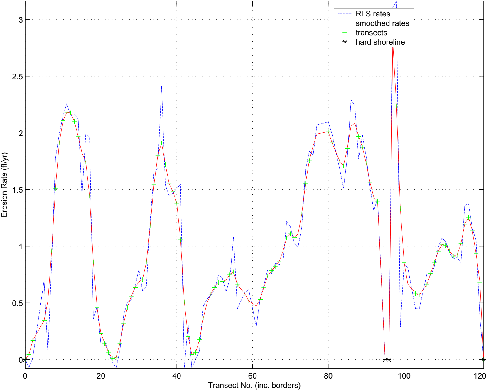
Calculated and Smoothed North Wailea Erosion Rates
