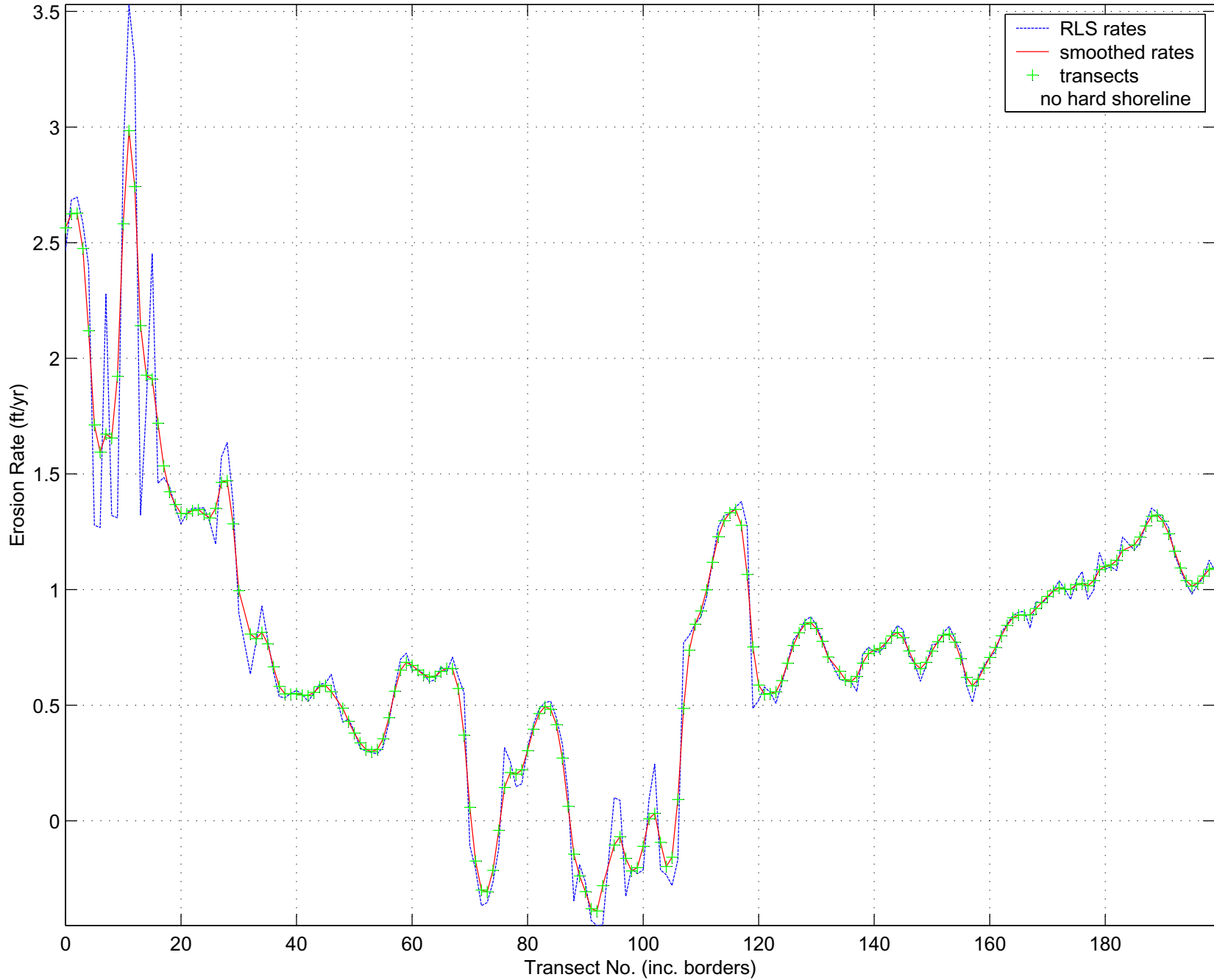
Calculated and Smoothed North Kihei Erosion Rates
