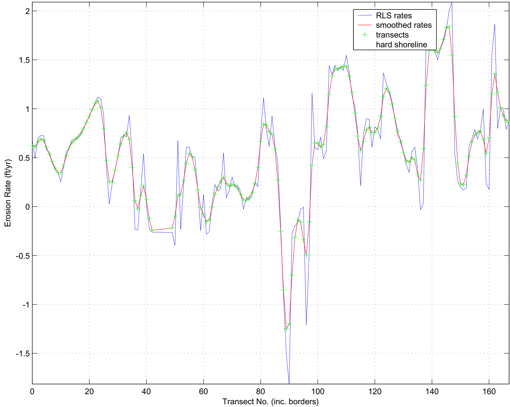
Calculated and Smoothed Launiupoko Erosion Rates
