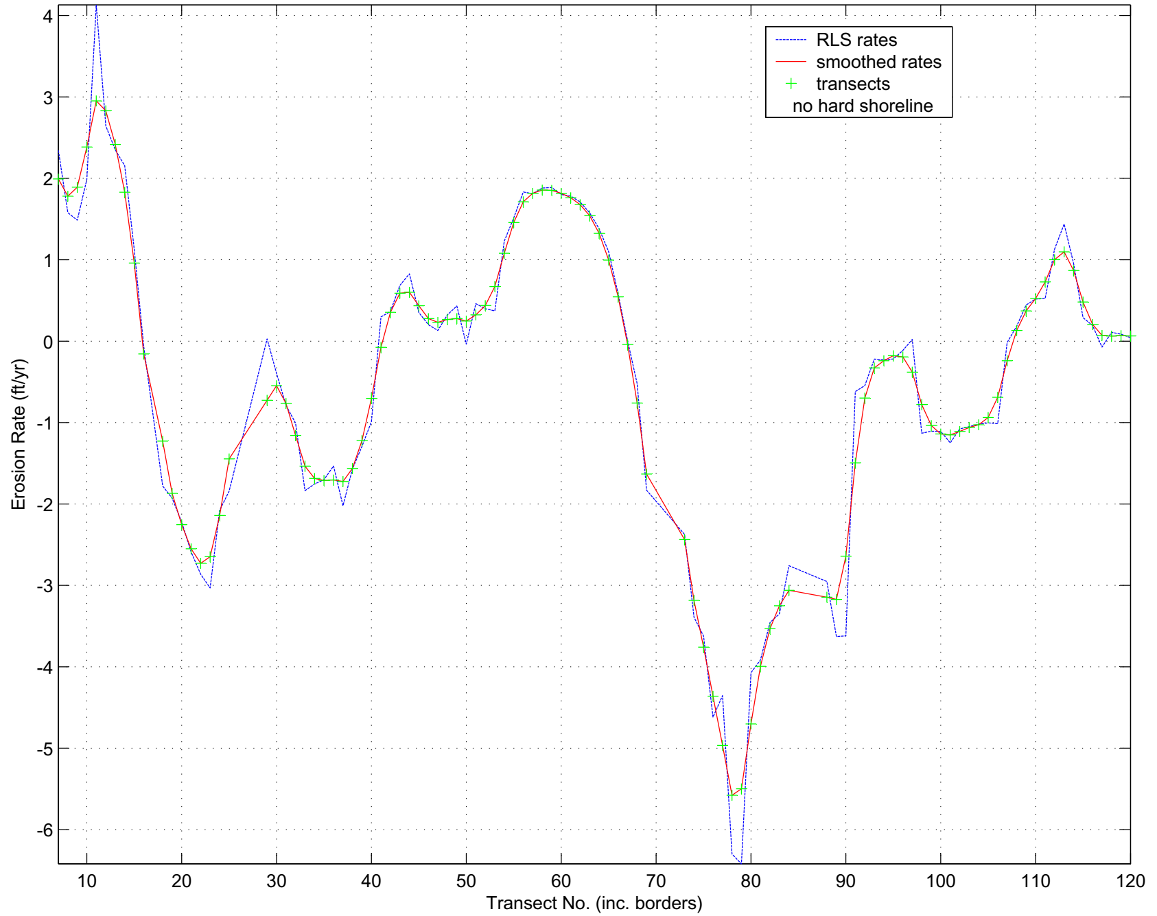
Calculated and Smoothed Kawililipoa Erosion Rates
