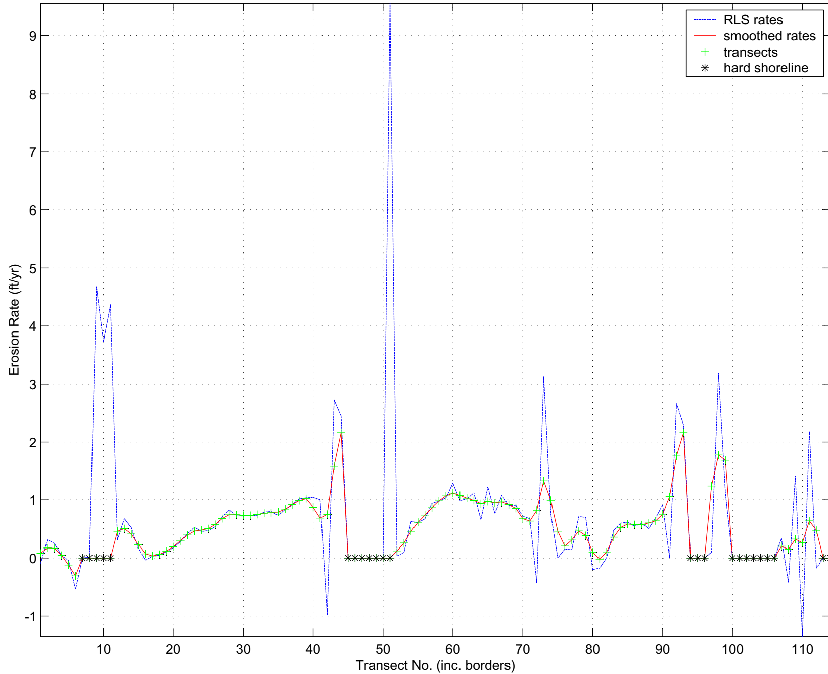
Calculated and Smoothed Kamaole Erosion Rates
