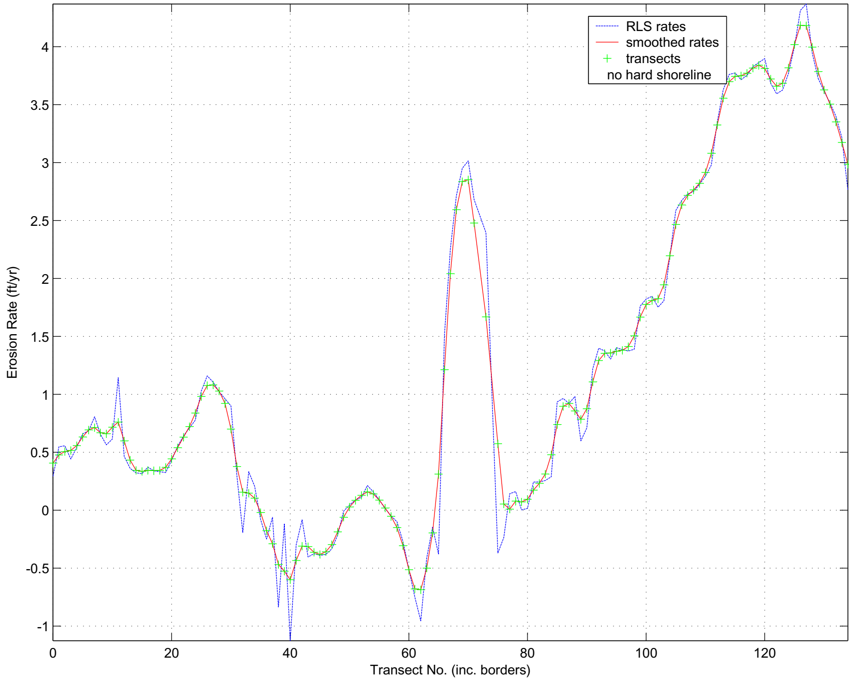
Calculated and Smoothed Kahului Harbor Erosion Rates
