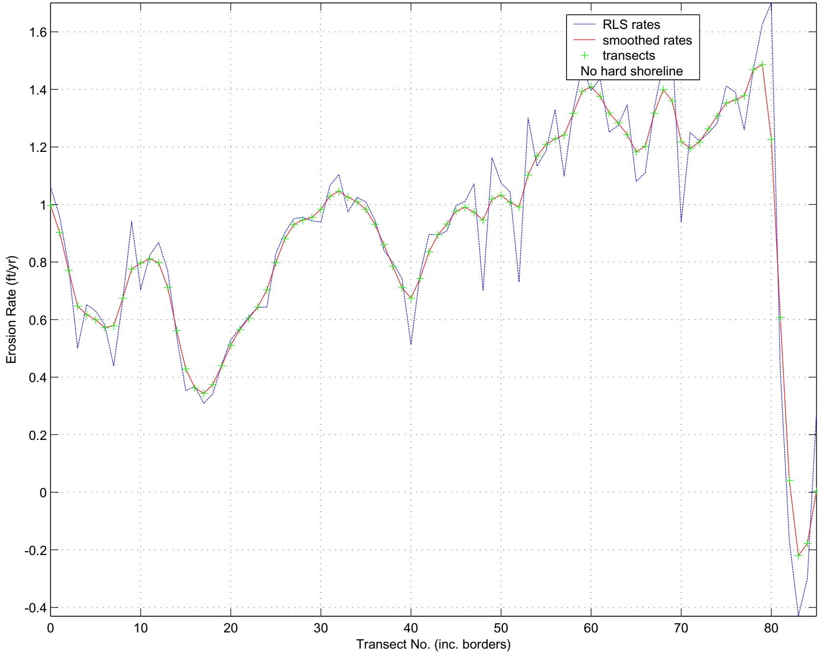
Calculated and Smoothed Honokowai Erosion Rates
