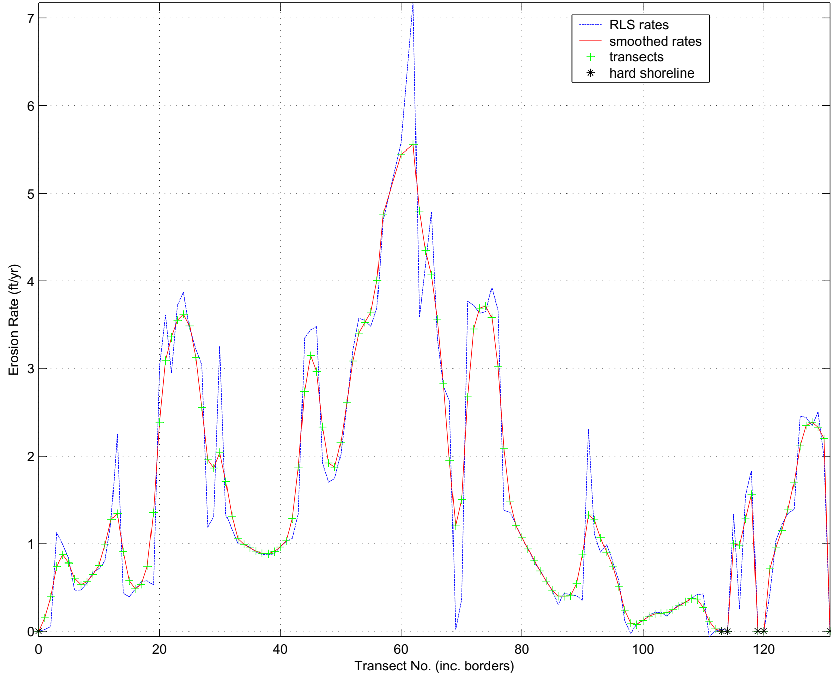
Calculated and Smoothed Baldwin Park Erosion Rates
