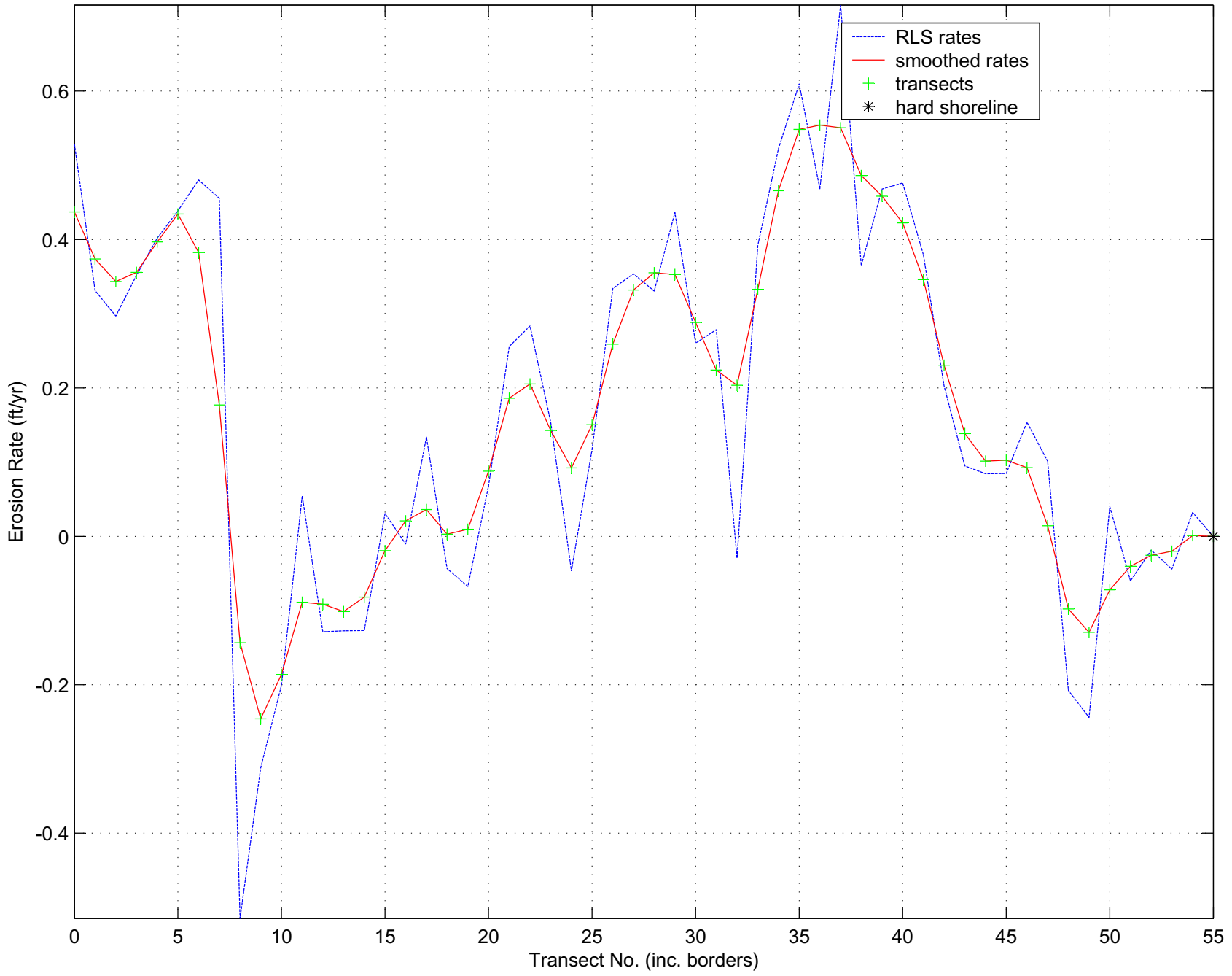
Calculated and Smoothed Awalua Erosion Rates
