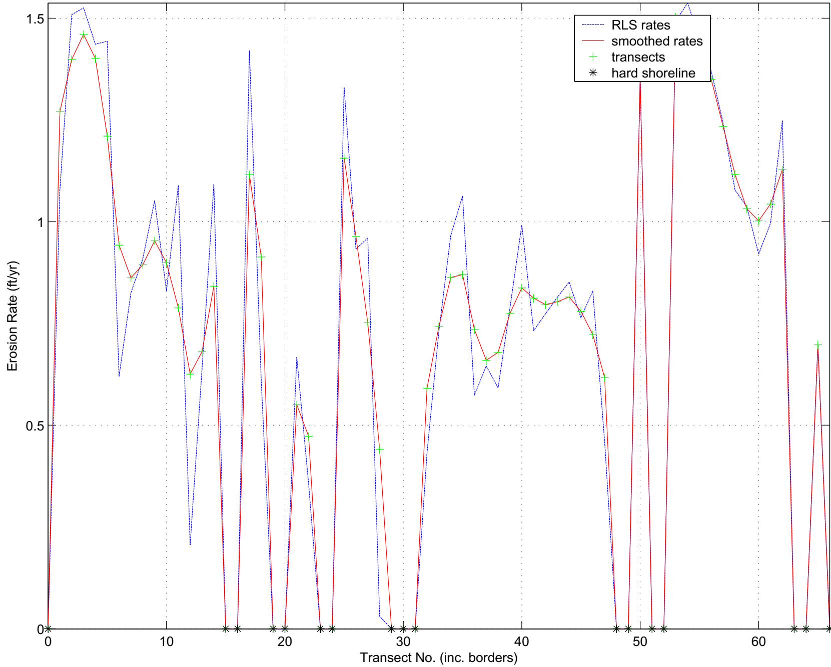
Calculated and Smoothed Alaaloa Erosion Rates
