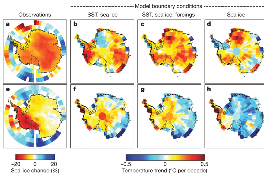
Figure 4 | Comparison of reconstructed and modelled mean annual temperature trends (degrees Celsius per decade) for the periods 1957–1981 and 1979–2003. a–d, 1957–1981; e–h, 1979–2003.
