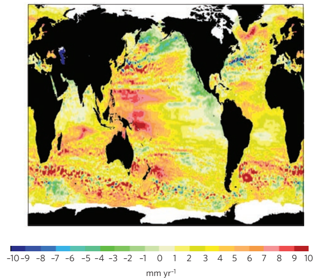
Figure 1 | Mean rate of sea-surface height change during October 1992 to May 2007, determined from satellite altimetry measurements.
