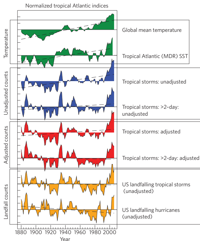
Figure 2 | Tropical Atlantic indices. Green-shaded curves depict global mean temperature (HadCRUT3 data set) and August–October main development region (MDR; 10^\circ \text{ N} – 20^\circ \text{ N} , 80^\circ \text{ W} – 20^\circ \text{ W} ) SST anomalies (HadISST data set). Blue-shaded curves represent unadjusted tropical storm counts. Red-shaded curves include time-dependent adjustments for missing storms based on ship-track density 20,22 . The curve labelled '>2-day' depicts storms with a duration greater than 2.0 days 22 . Orange-shaded curves depict US landfalling tropical storms and hurricanes (no adjustments). Solid black lines are five-year means (1878–2008); dashed black lines are linear trends. Vertical axis ticks represent one standard deviation. Series normalized to unit standard deviation. Only the top three series have significant linear trends ( p = 0.05 ). Figure reproduced with permission from refs 20 (© 2008 AMS) and 22 (© 2009 AMS).
